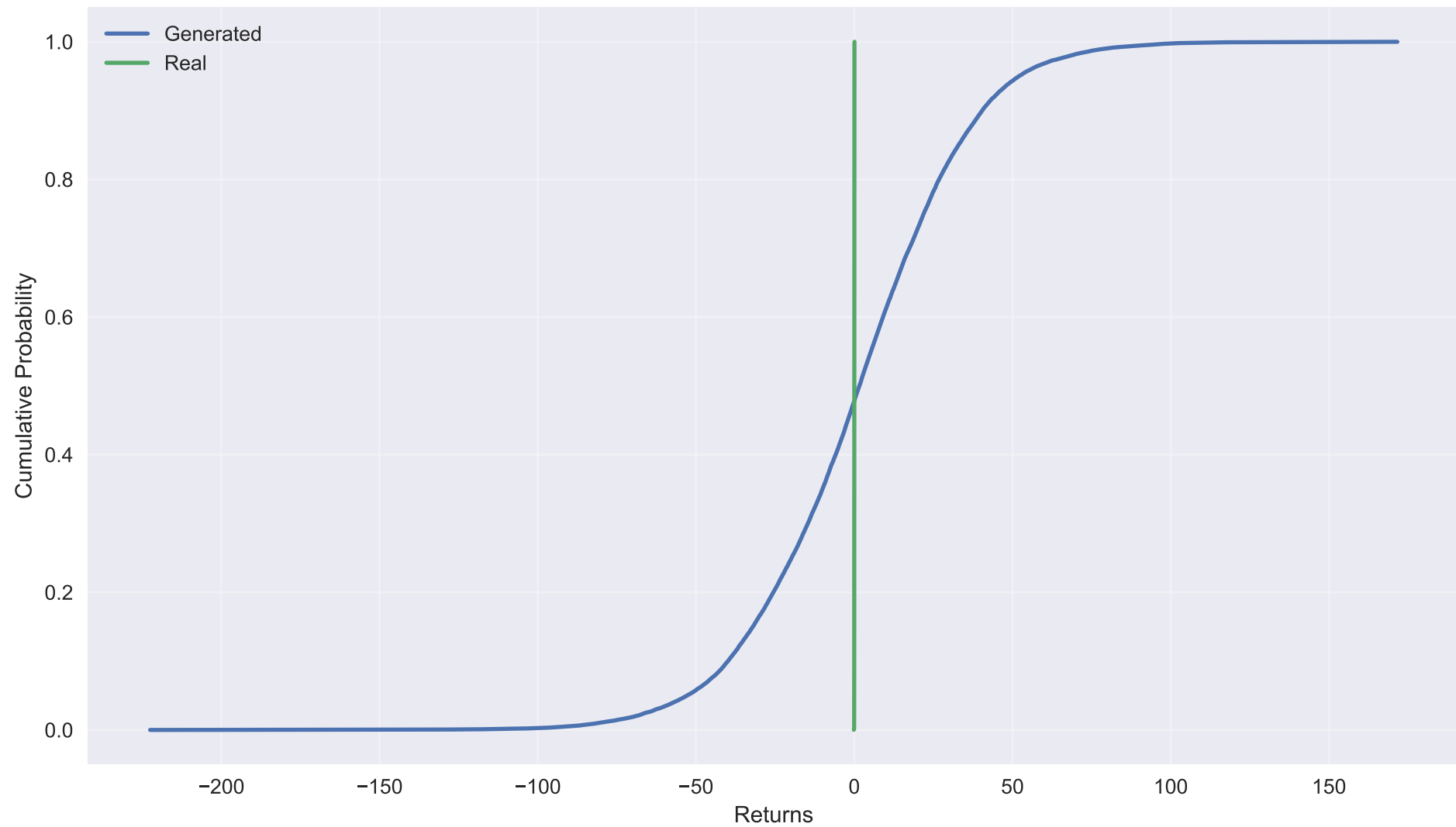
Llm Conditioned: ECDF Comparison
